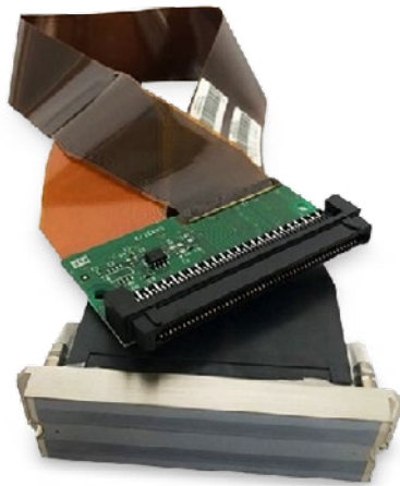
RICOH PrinterHead
